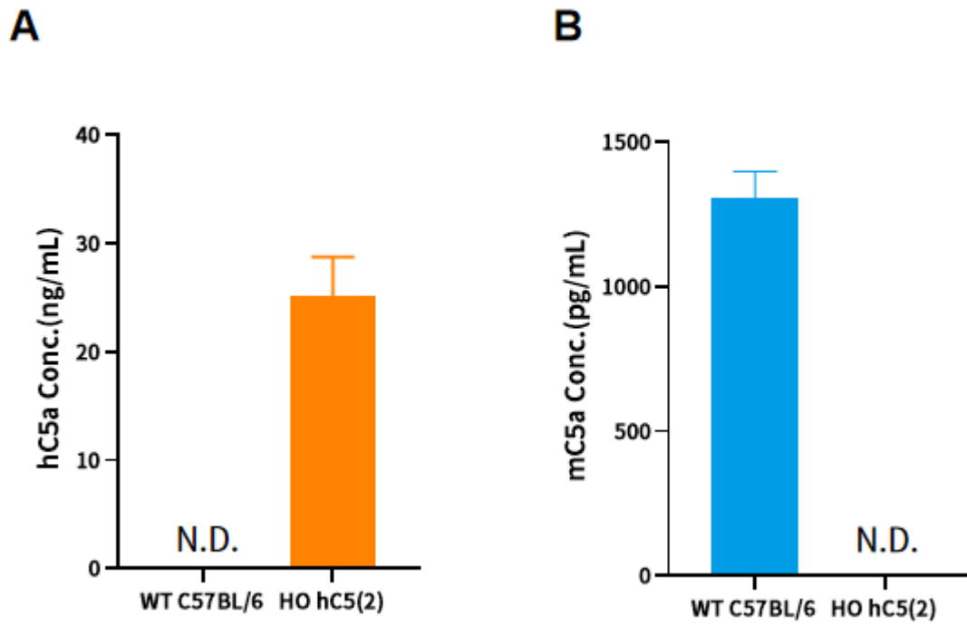
Fig.1 Detection of hC5a and mC5a expression in serum by ELISA.
